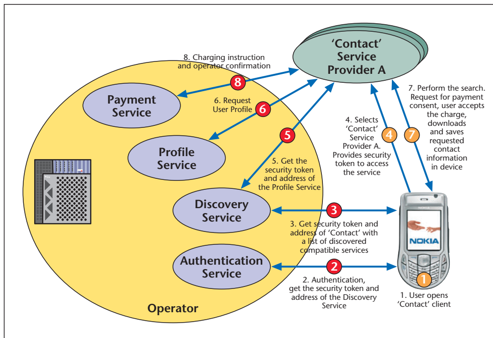
Figure 9. Contact search with multiple Service Provider options
